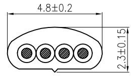
SECTION: A-A SCALE 4:1
